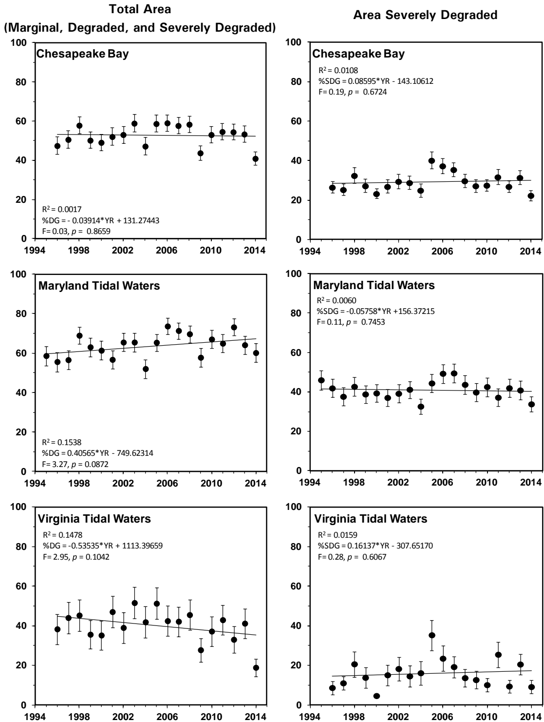
Figure 3-31. Proportion of the Chesapeake Bay, Maryland tidal waters, and Virginia tidal waters failing the Chesapeake Bay benthic community restoration goals, 1996 to 2014 (1995-2014 for Maryland). Panels on left show percent total area degraded (B-IBI < 3.0); panels on right show percent area severely degraded (B-IBI ≤ 2.0). Error bars indicate ± 1 SE. The mainstem deep trough is included in the severely degraded condition estimates
