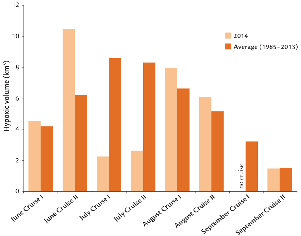
Figure 3-36. Hypoxic volume in Chesapeake Bay in 2014 compared to the long-term average. Source: EcoCheck , University of Maryland Center for Environmental Science (UMCES). Data provided by Maryland DNR and Virginia DEQ.
