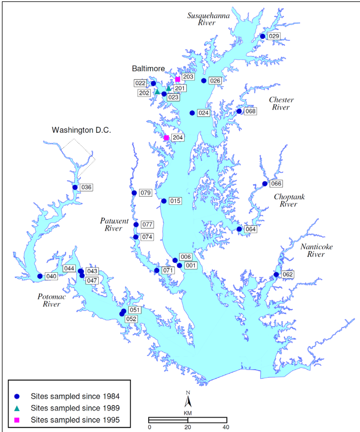
Figure 2-1. Fixed sites sampled in 2014
