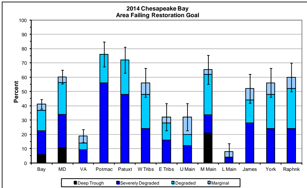
Figure 3-34. Proportion of the Chesapeake Bay, Maryland, Virginia, and the 10 sampling strata failing the Chesapeake Bay benthic community restorations goals in 2014. Error bars indicate \pm 1 SE
