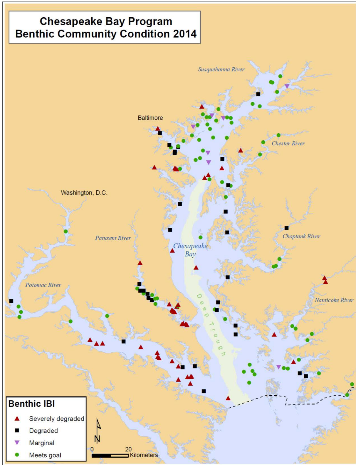
Figure 3-29. Results of probability-based benthic sampling of the Maryland Chesapeake Bay and its tidal tributaries in 2014. Each sample was evaluated in context of the Chesapeake Bay benthic community restoration goals
