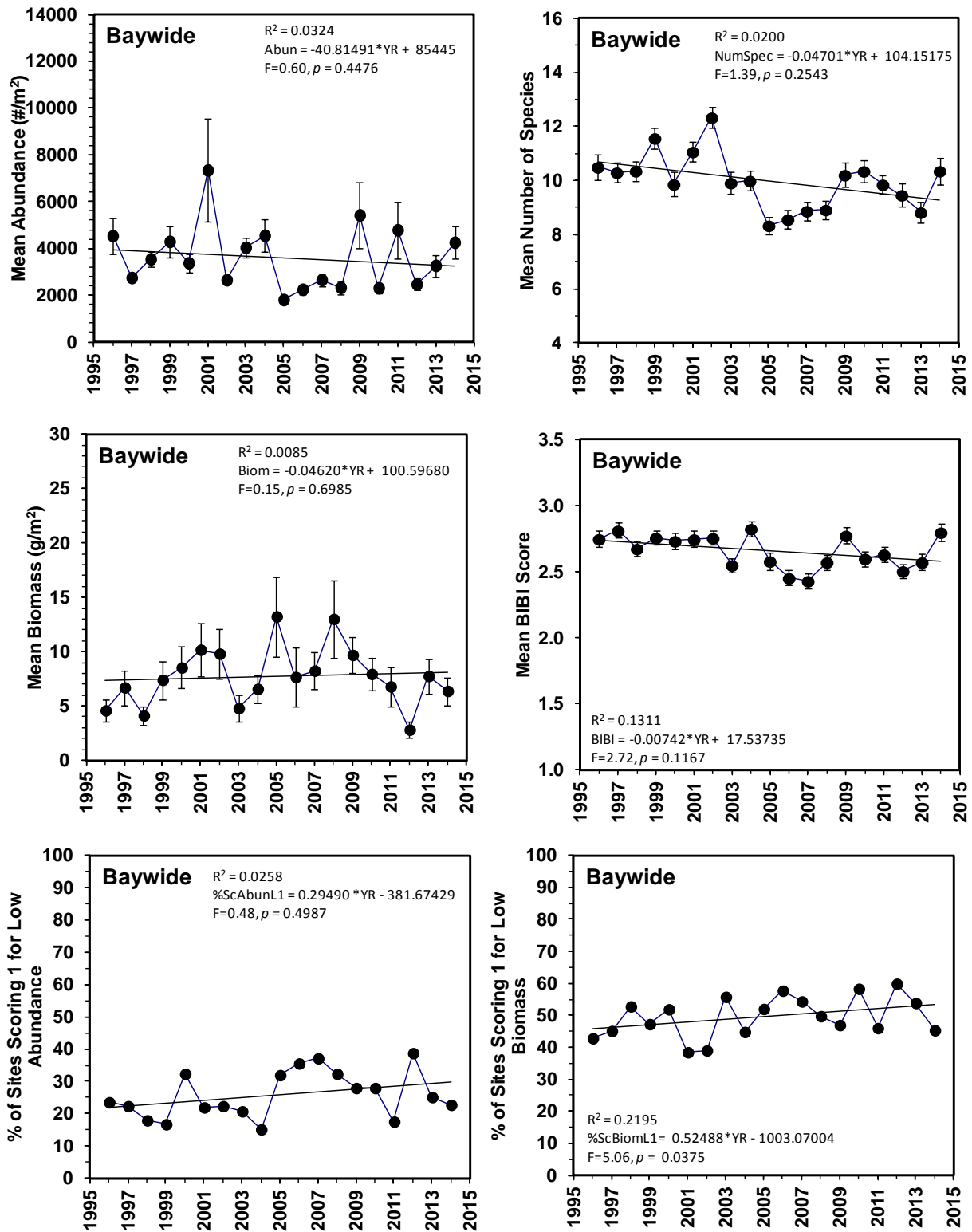
Figure 3-38. Trends in abundance, biomass, number of species, B-IBI (mean \pm 1 SE), and percent sites scoring "1" for low abundance or low biomass in Chesapeake Bay, 1996-2014 (N = 250 sites per year)
