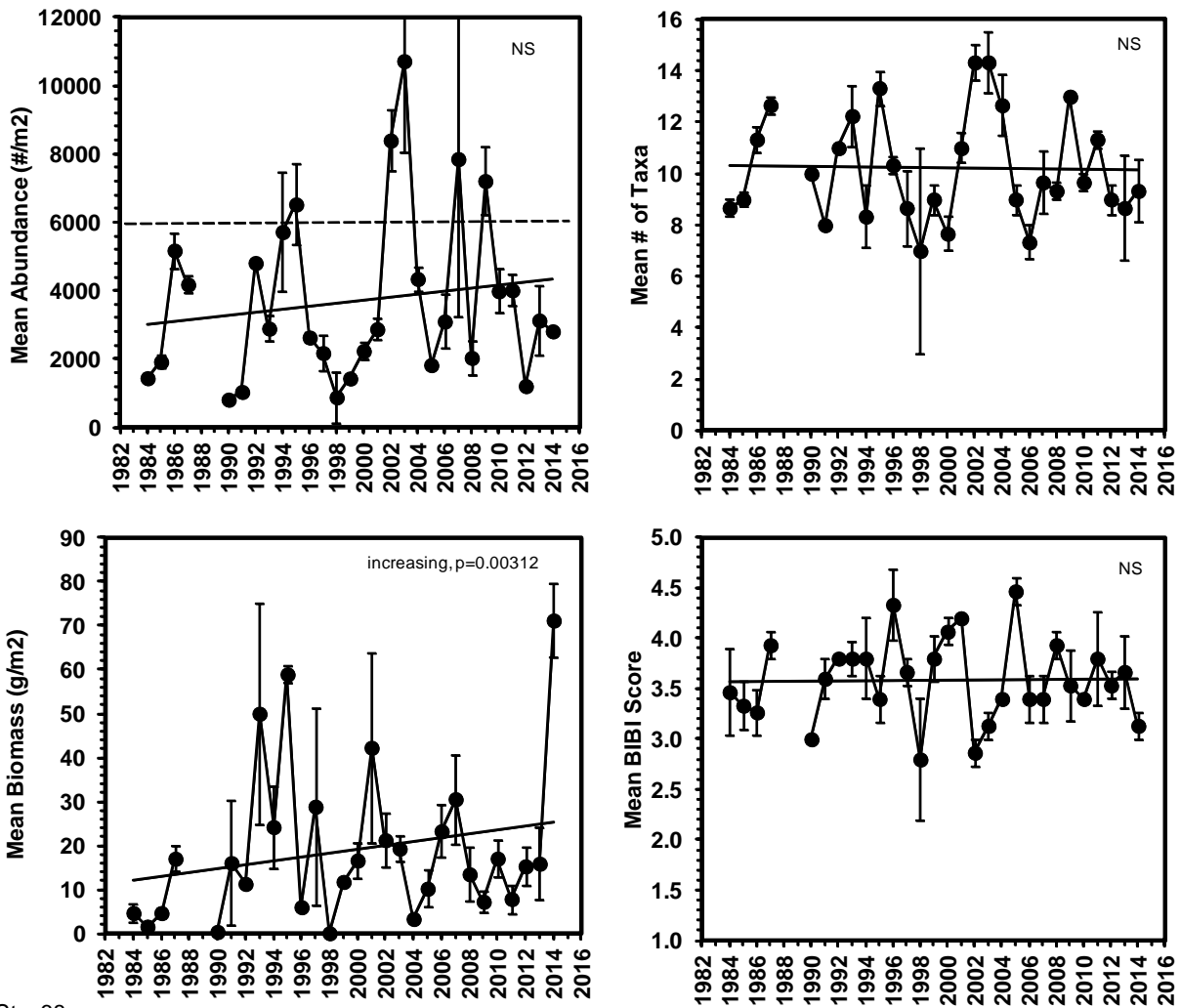
Figure 3-19. Trends in abundance, biomass, number of species, and B-IBI (mean ± 1 SE) at fixed sites. Station 68 = Chester River. The dashed line in the abundance plot is the upper B-IBI threshold (scored as 1) for abundance
