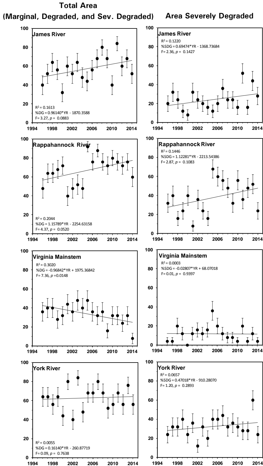
Figure 3-33. Proportion of the Virginia sampling strata failing the Chesapeake Bay benthic community restoration goals, 1996 to 2014. Panels on left show percent total area degraded (B-IBI < 3.0); panels on right show percent area severely degraded (B-IBI ≤ 2.0). Error bars indicate ± 1 SE
