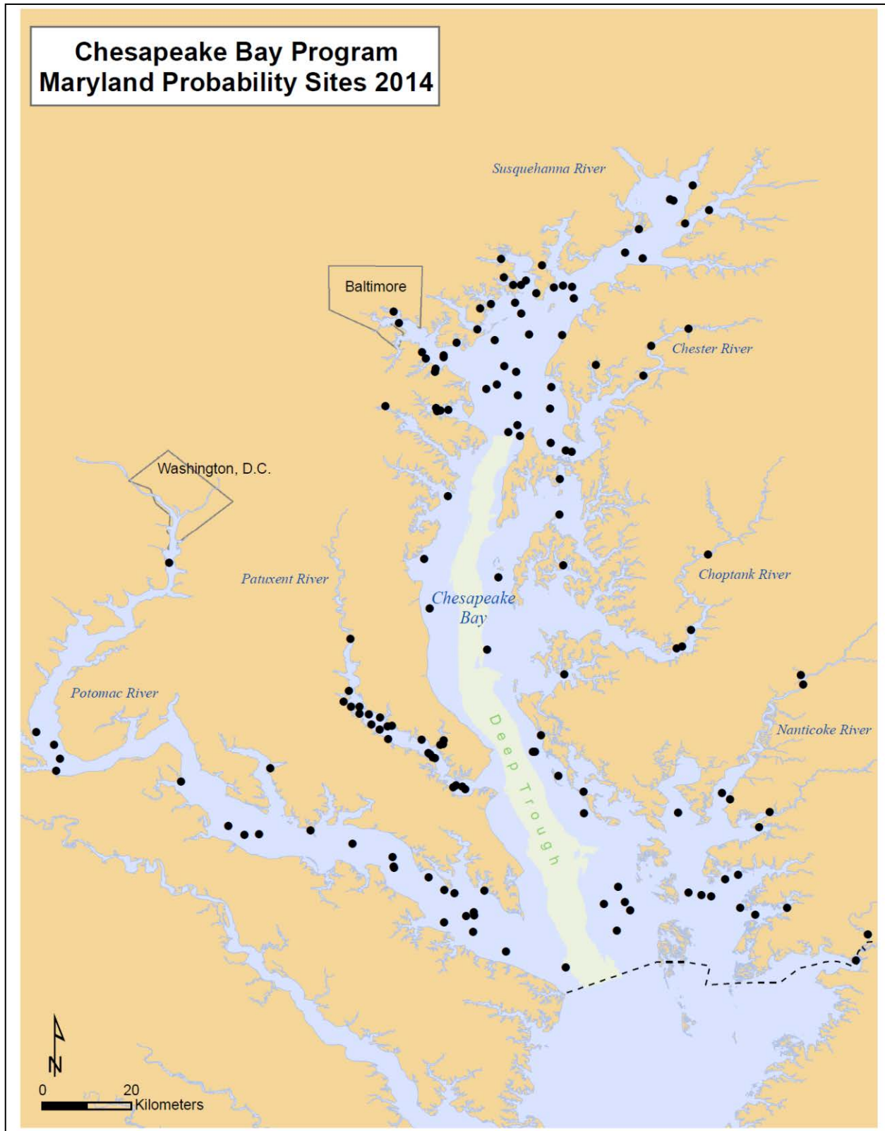
Figure 2-5. Maryland probability-based sampling sites for 2014
