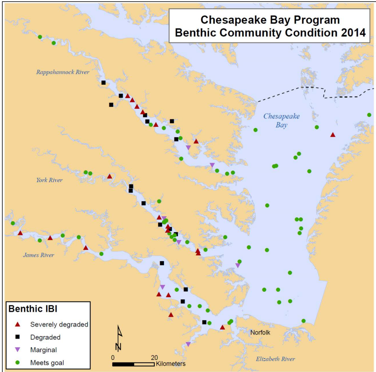
Figure 3-30. Results of probability-based benthic sampling of the Virginia Chesapeake Bay and its tidal tributaries in 2014. Each sample was evaluated in context of the Chesapeake Bay benthic community restoration goals
