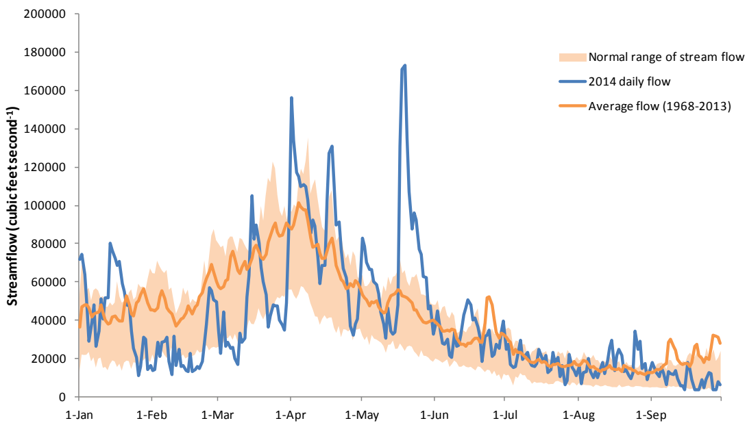
Figure 3-35. Daily flow entering the Chesapeake Bay from the Susquehanna River at Conowingo in 2013 (top panel) and 2014 (bottom panel), compared to the long-term average. Normal range of stream flow: 25%-75%. Data source: United States Geological Survey
