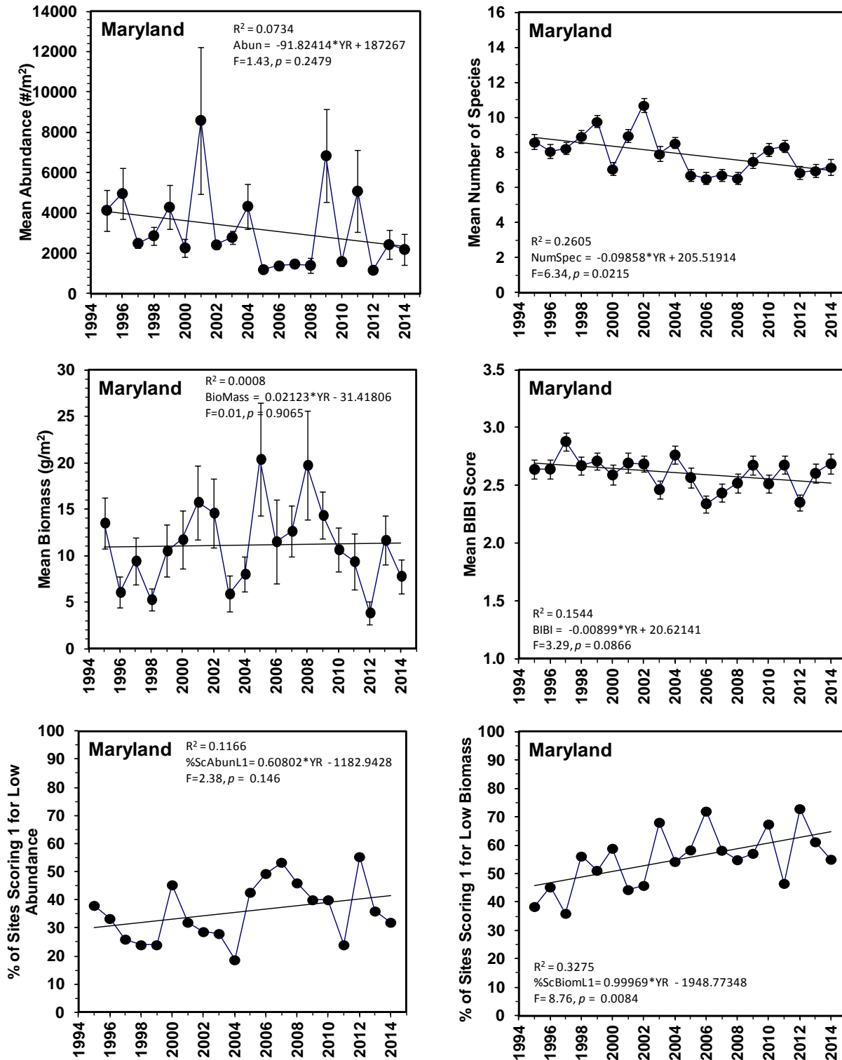
Figure 3-37. Trends in abundance, biomass, number of species, B-IBI (mean \pm 1 SE), and percent sites scoring "1" for low abundance or low biomass in Maryland tidal waters, 1995-2014 (N = 150 sites per year)
