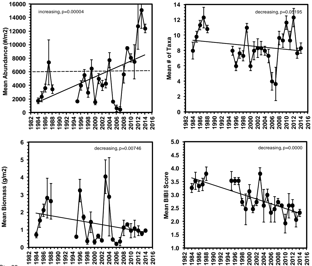
Figure 3-16. Trends in abundance, biomass, number of species, and B-IBI (mean ± 1 SE) at fixed sites. Station 62 = Nanticoke River. The dashed line in the abundance plot is the upper B-IBI threshold (scored as 1) for abundance
