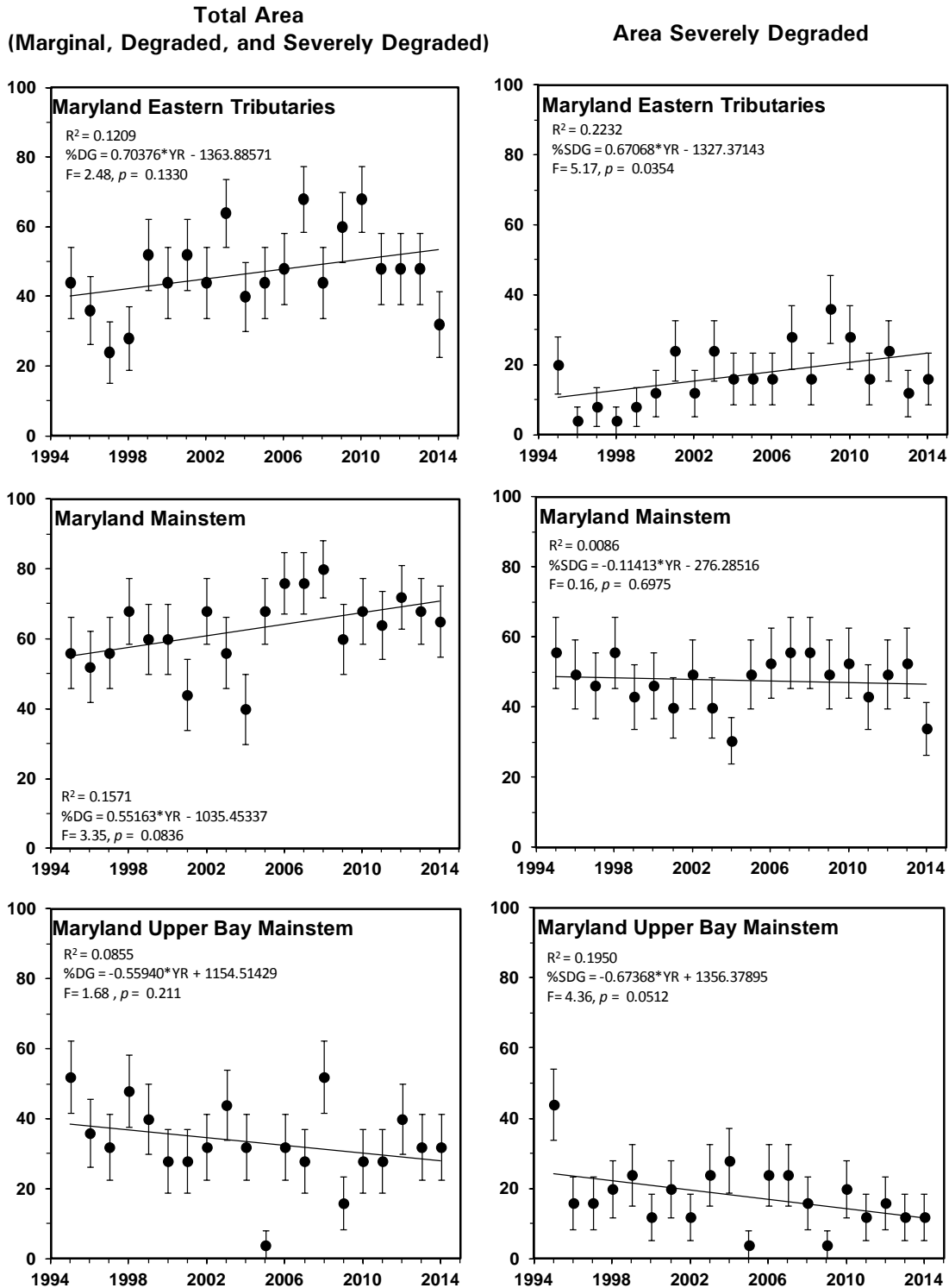
Figure 3-32. Proportion of the Maryland sampling strata failing the Chesapeake Bay benthic community restoration goals, 1995 to 2014. Panels on left show percent total area degraded (B-IBI < 3.0); panels on right show percent area severely degraded (B-IBI ≤ 2.0). Error bars indicate ± 1 SE. The deep trough is included in the Maryland mainstem stratum estimates
