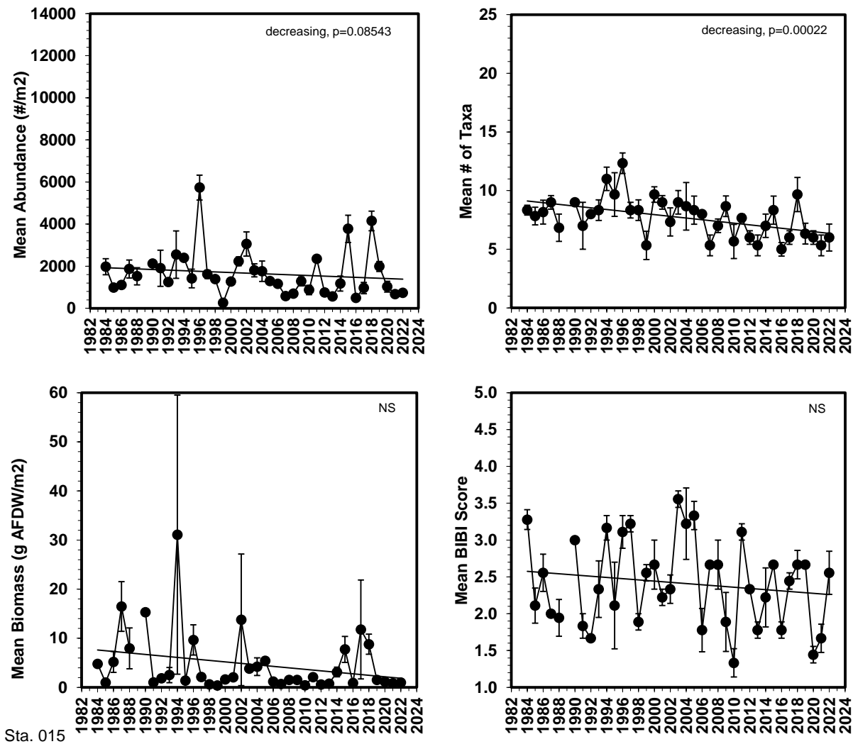
Figure 3-4. Trends in abundance, biomass, number of species, and B-IBI (mean \pm 1 SE) at fixed sites. Station 015 = Chesapeake mainstem ( \leq 5 m), North Beach. Data gaps indicate periods where sampling was suspended because of program design changes
