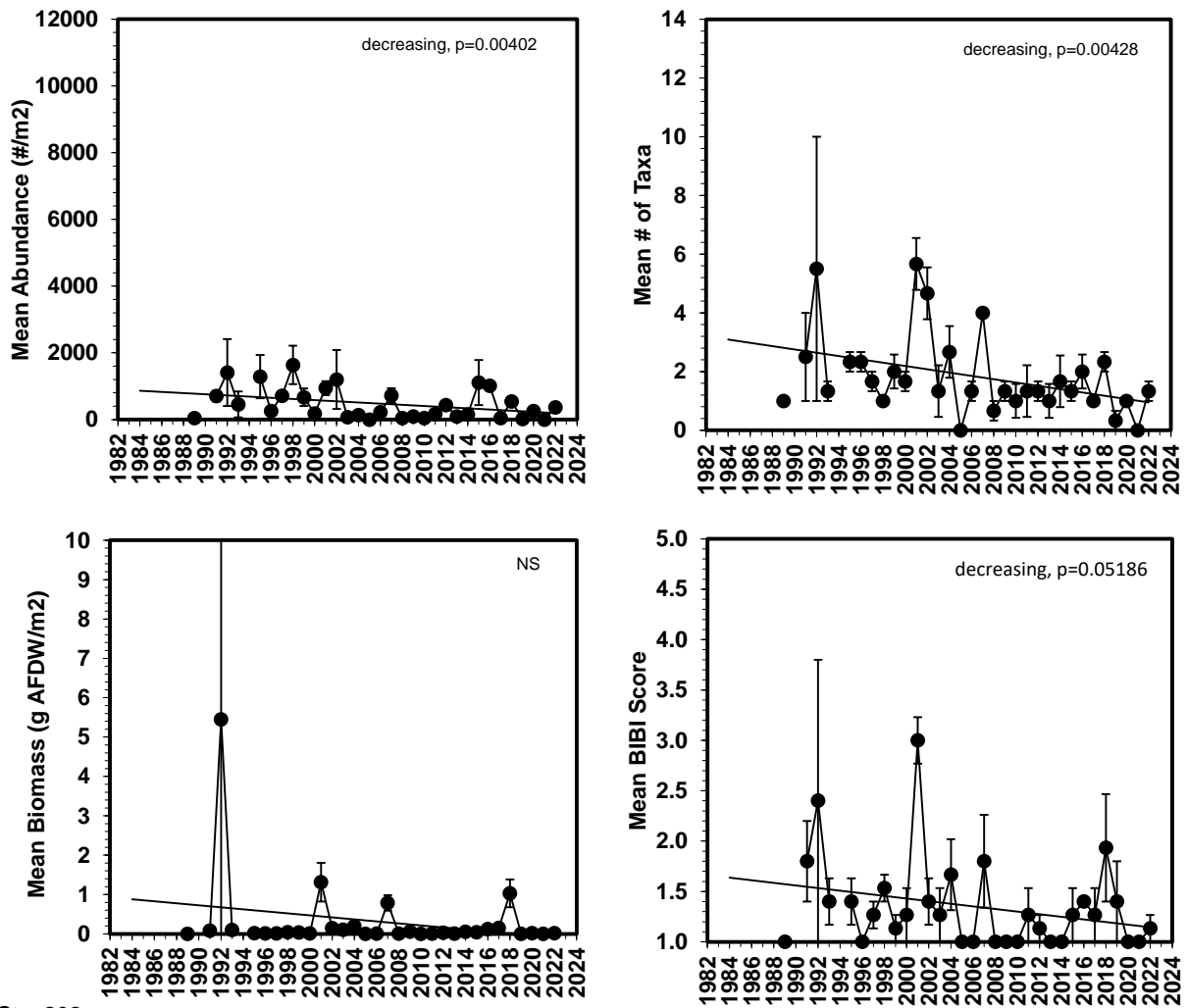
Figure 3-26. Trends in abundance, biomass, number of species, and B-IBI (mean \pm 1 SE) at fixed sites. Station 202 = Patapsco River estuary, Curtis Creek. Data gaps indicate periods where sampling was suspended because of program design changes
