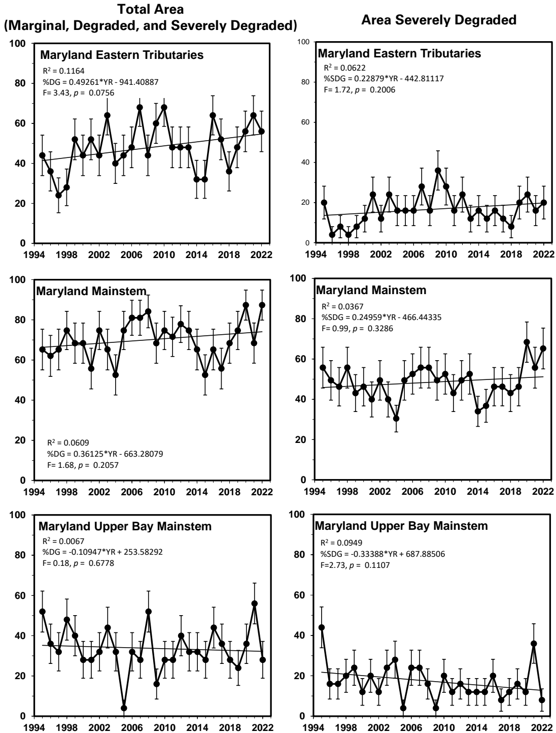
Figure 3-33. Proportion of the Maryland sampling strata failing the Chesapeake Bay benthic community restoration goals, 1995 to 2022. Panels on left show percent total area degraded (B-IBI<3); panels on right show percent area severely degraded (B-IBI≤2). Error bars indicate ± 1 standard error. The deep trough is included in the Maryland mainstem stratum estimates. See cautionary note in page 3-37
